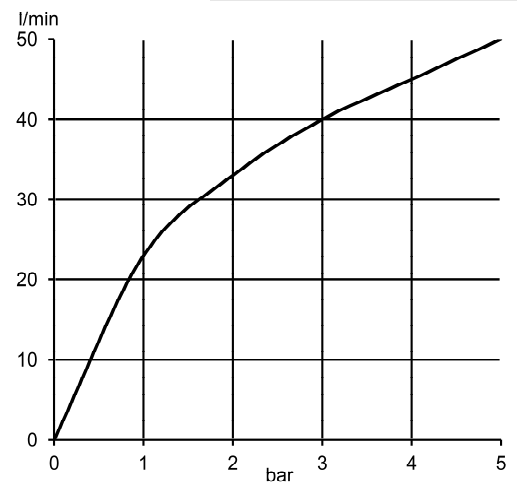
Flow rate diagramm
