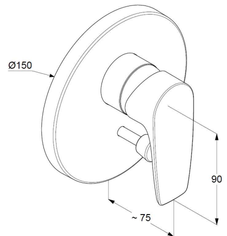
Dimensional drawing
